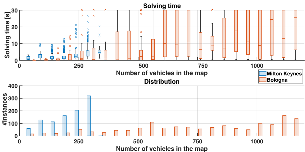
Figure 4: (Top) Boxplot of the solving time of CLINGO in correlation with the number of vehicles inside the networks. (Bottom) Histogram representing the number of instances (i.e., each time a new vehicle enters the network) w.r.t. the number of vehicles inside the map. In the two charts, the x-axis has been clustered in bins of 50.
